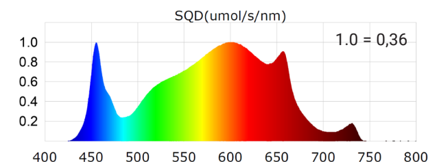
fig. 1: Actual emission spectrum measured with Everfine SP20 Suite (wavelength in nm vs. power in µmol/s)
